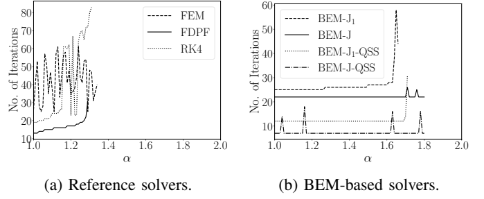
Fig. 7: Iterations of \theta_{bus2} for all methods, \alpha \in (1, 2] .
