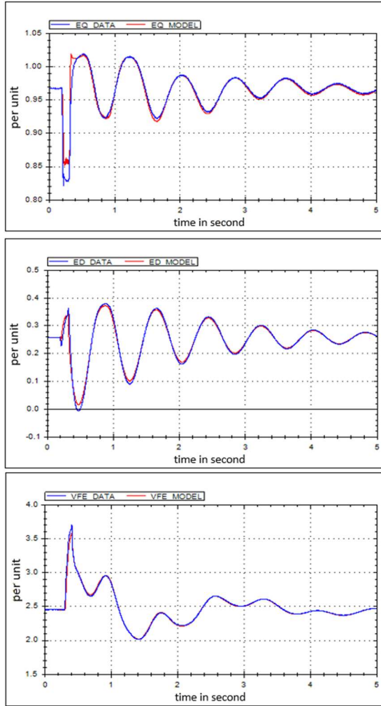
Figure 5. Depiction of a triggering event and parameter estimation due to a three-phase fault in the simulated system.
