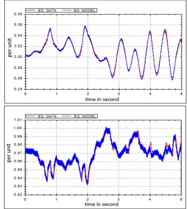
Figure 3. Comparison of the d-q axis voltages.
