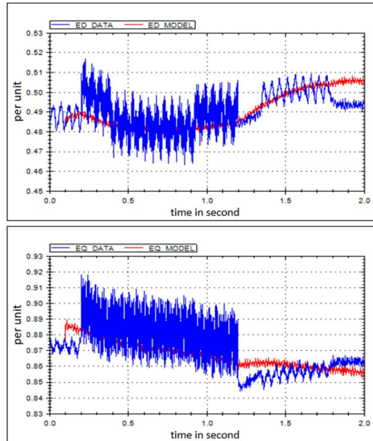
Figure 6. Depiction of a simulated intermittent stator fault of 20% from the neutral triggering the data log and parameter estimation.
