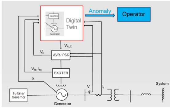
Figure 2. Model validation of a power plant.
