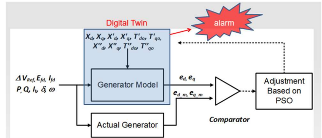
Figure 1. Detection of an anomaly of in the generating system.
