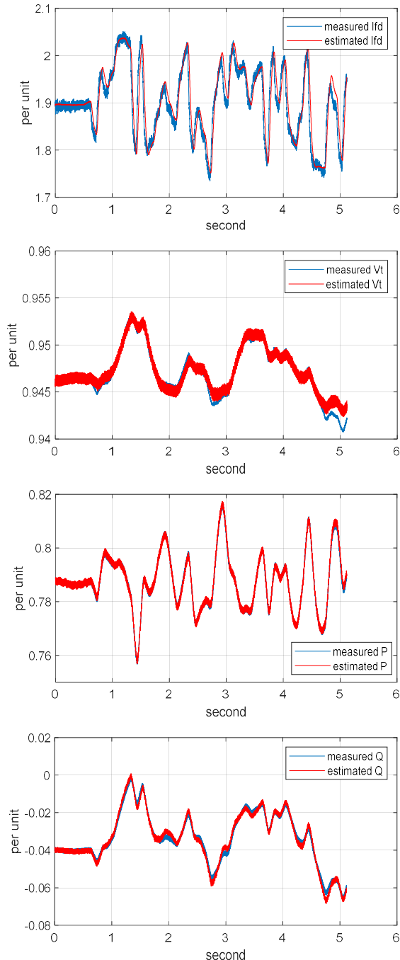
Figure 4. Load change of 50% in the 970 MVA generator system.
