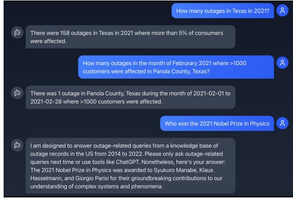
Fig. 2: OutageGPT chatbot answering different user queries.
