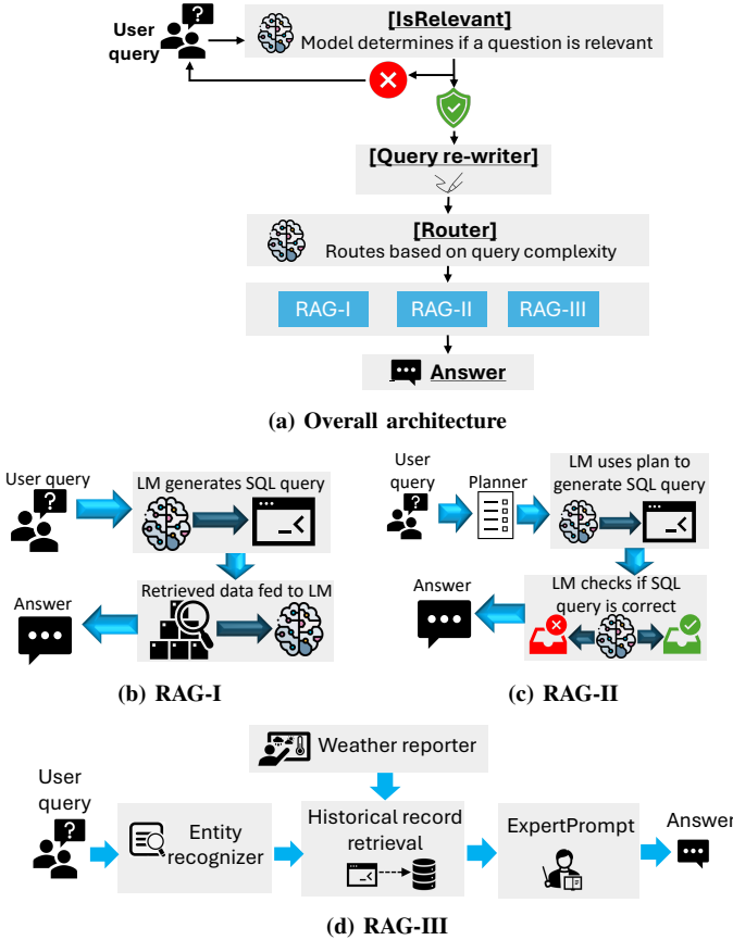
Fig. 1: Architecture of our proposed multi-agent RAG model.
