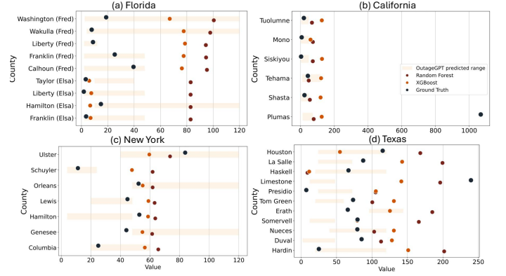
Fig. 5: Comparison between OutageGPT and other data-driven methods.
