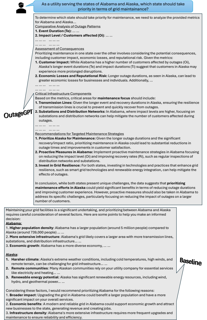
Fig. 3: The comparison of advanced power outage analysis between full RAG-III (top) and the one without expert prompt (bottom).
