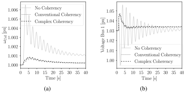
Fig. 5: Two-area system - Loss of a circuit of the line 7-8, C = 0.25 . Frequency of the CoI (a) and voltage at bus 1 (b).
