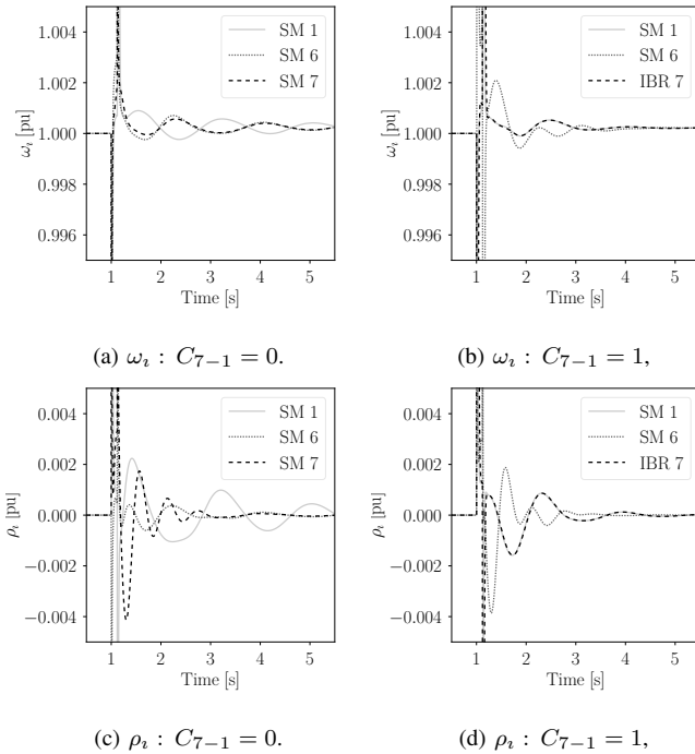
Fig. 7: IEEE 39-Bus system – Three phase fault at bus 1 - real and imaginary parts of the CF of the current of generators 1, 6, and 7 for C_{7-1} = 0 and C_{7-1} = 1 .
